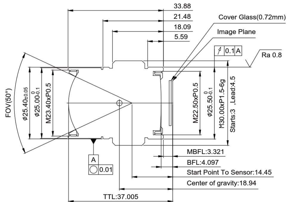
2D outline
